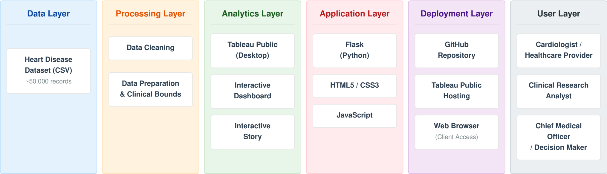
Figure 1: Technical pipeline layout and data flow of the Heart Disease Analysis dashboard application.
